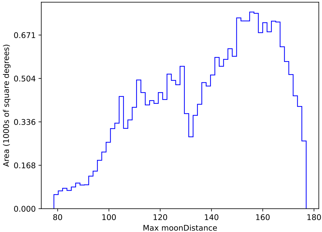
ddf_acor_sf10_lsf40_lsr10_v3.4_10yrs All sky y band: Max moonDistance
