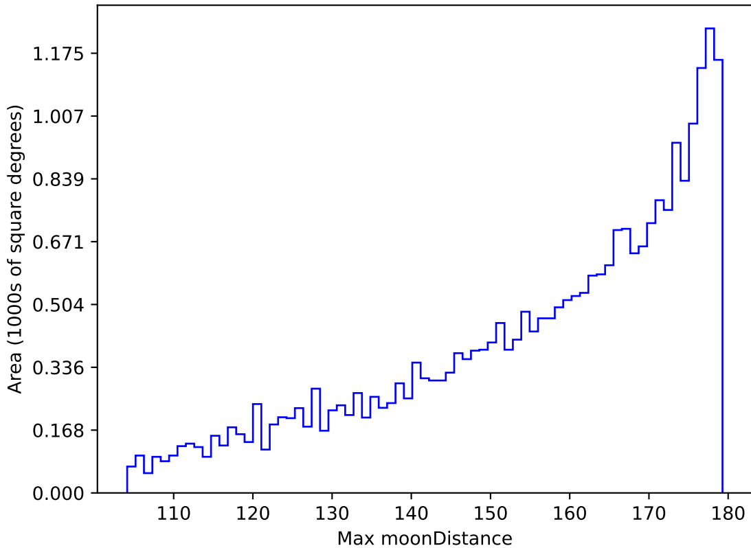
ddf_acor_sf10_lsf40_lsr10_v3.4_10yrs All sky r band: Max moonDistance
