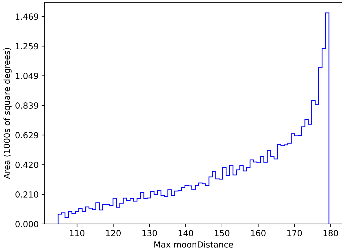
ddf_acor_sf10_lsf40_lsr10_v3.4_10yrs All sky all bands: Max moonDistance
