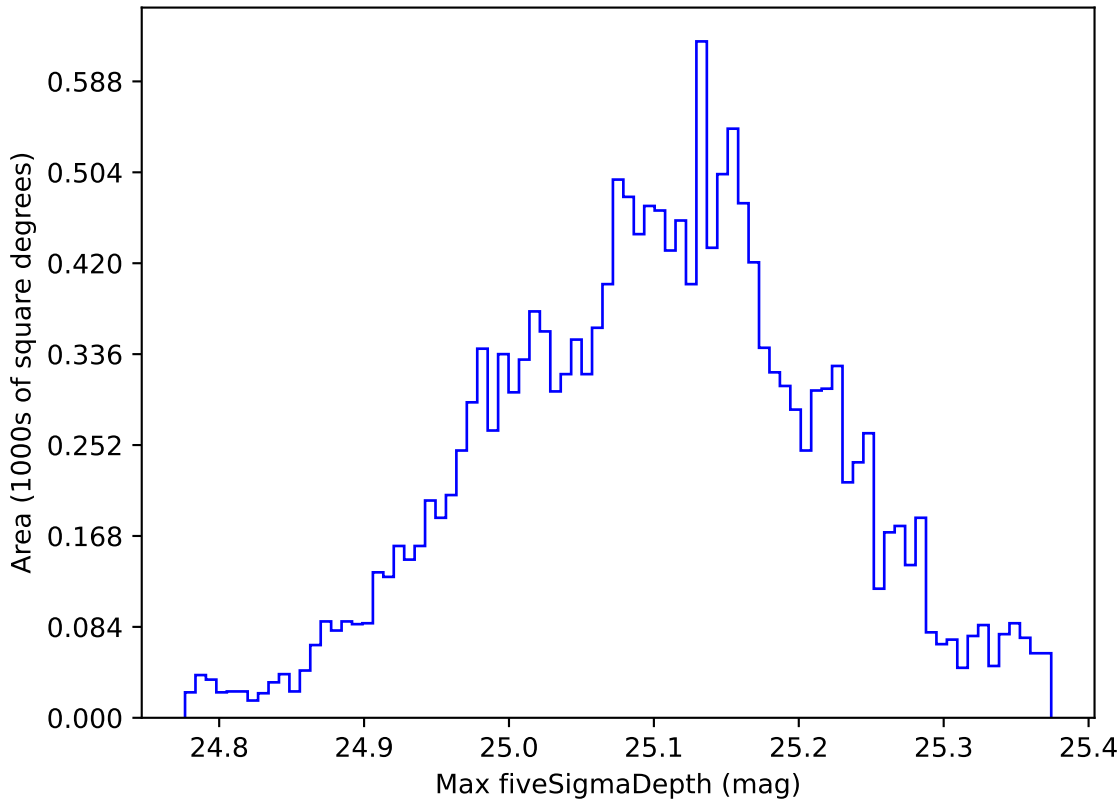
ddf_acor_sf10_lsf40_lsr10_v3.4_10yrs WFD all bands: Max fiveSigmaDepth
