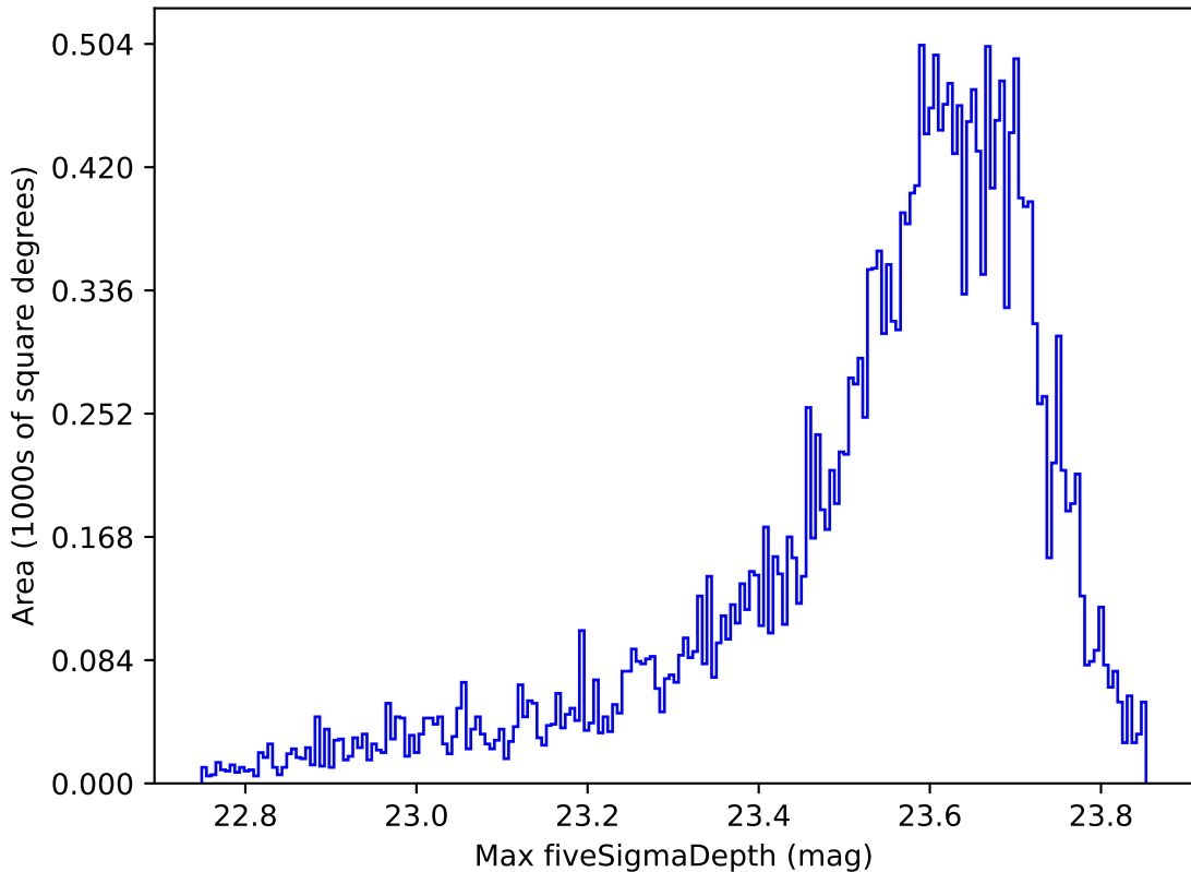
ddf_acor_sf10_lsf40_lsr10_v3.4_10yrs All sky z band: Max fiveSigmaDepth
