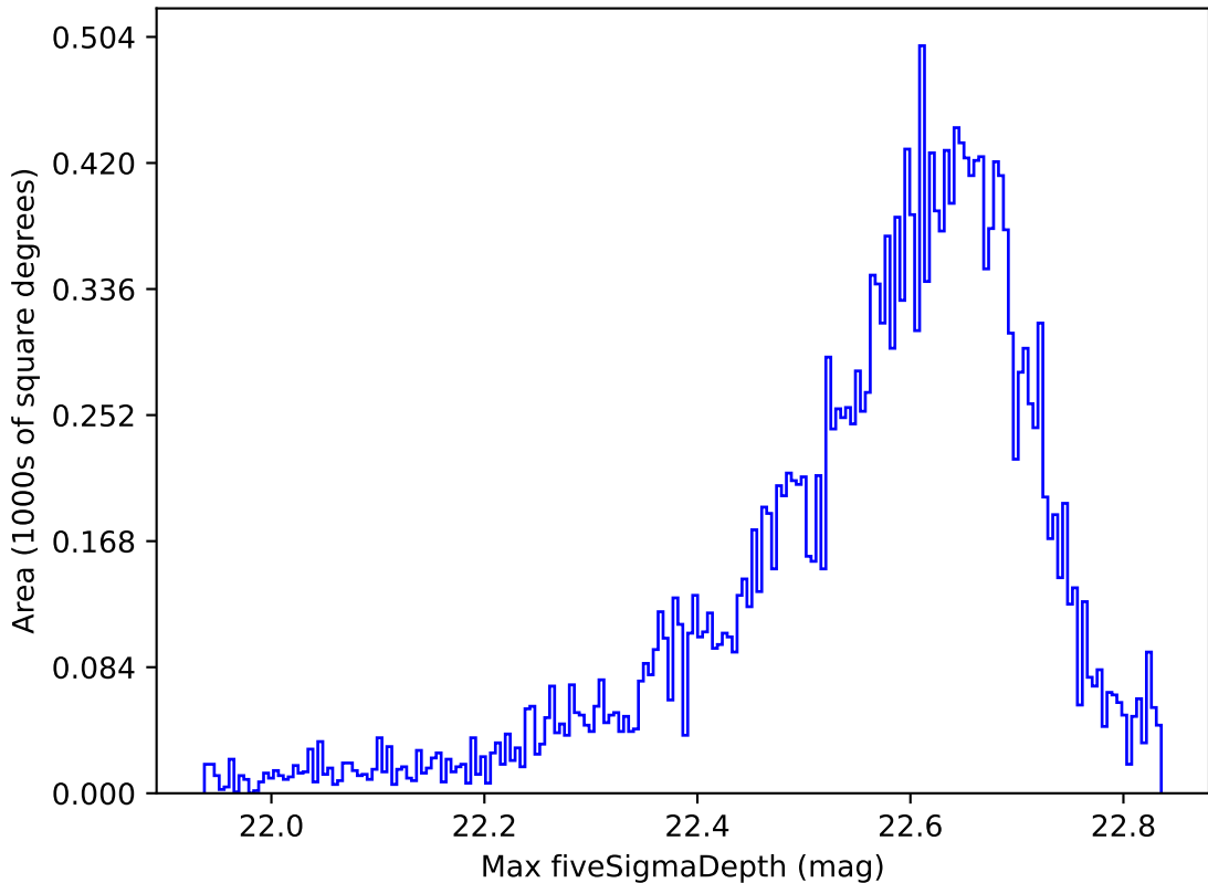
ddf_acor_sf10_ls40_lsr10_v3.4_10yrs All sky y band: Max fiveSigmaDepth
