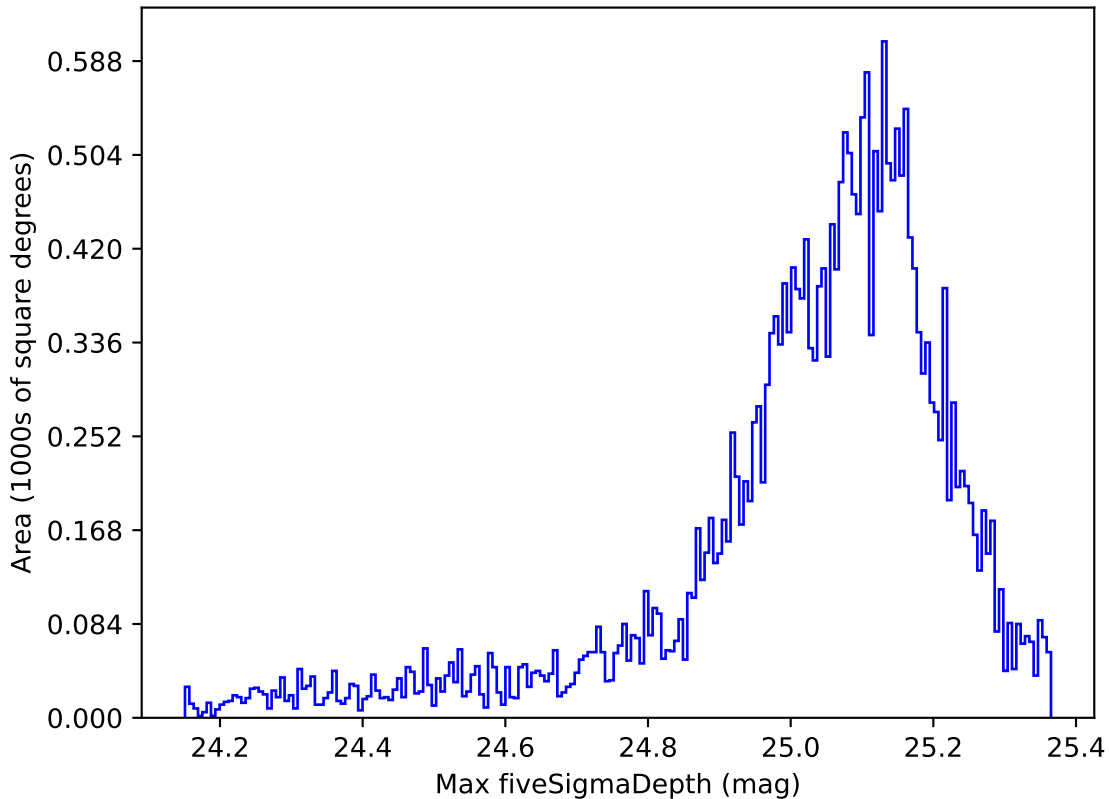
ddf_acor_sf10_ls40_lsr10_v3.4_10yrs All sky g band: Max fiveSigmaDepth
