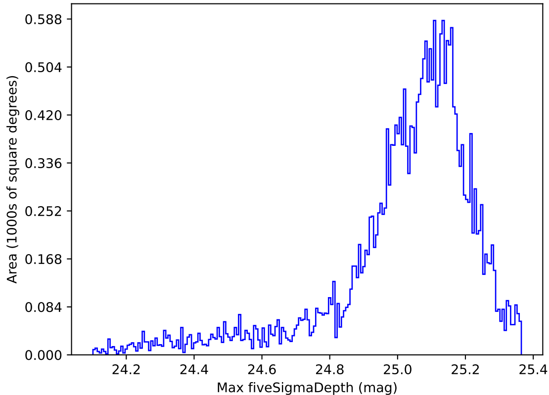
ddf_acor_sf10_lsf40_lsr10_v3.4_10yrs All sky all bands: Max fiveSigmaDepth
