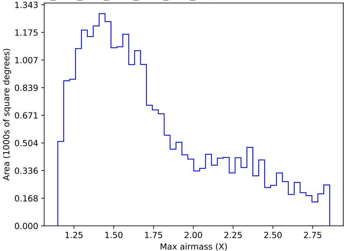
ddf_acor_sf10_lsf40_lsr10_v3.4_10yrs Yr 1 z band: Max airmass
