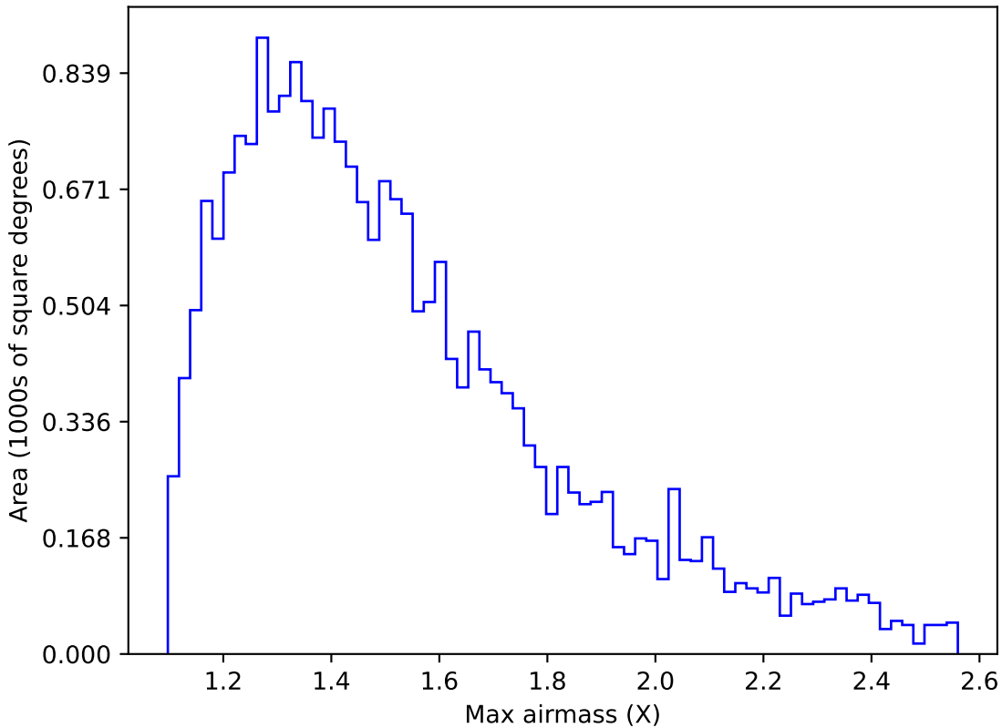
ddf_acor_sf10_lsf40_lsr10_v3.4_10yrs Yr 1 u band: Max airmass
