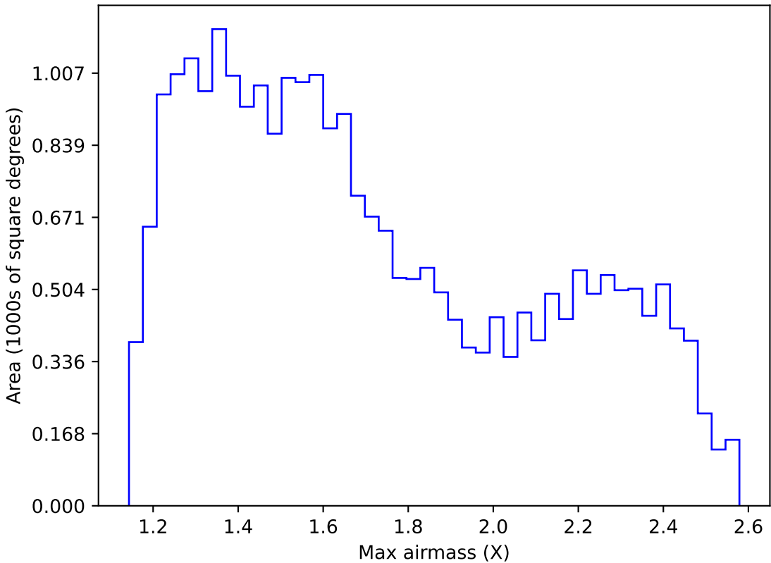
ddf_acor_sf10_lsf40_lsr10_v3.4_10yrs Yr 1 r band: Max airmass
