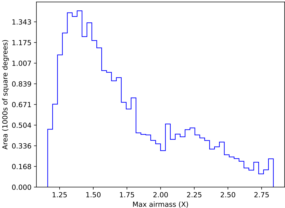
ddf_acor_sf10_lsf40_lsr10_v3.4_10yrs Yr 1 i band: Max airmass
