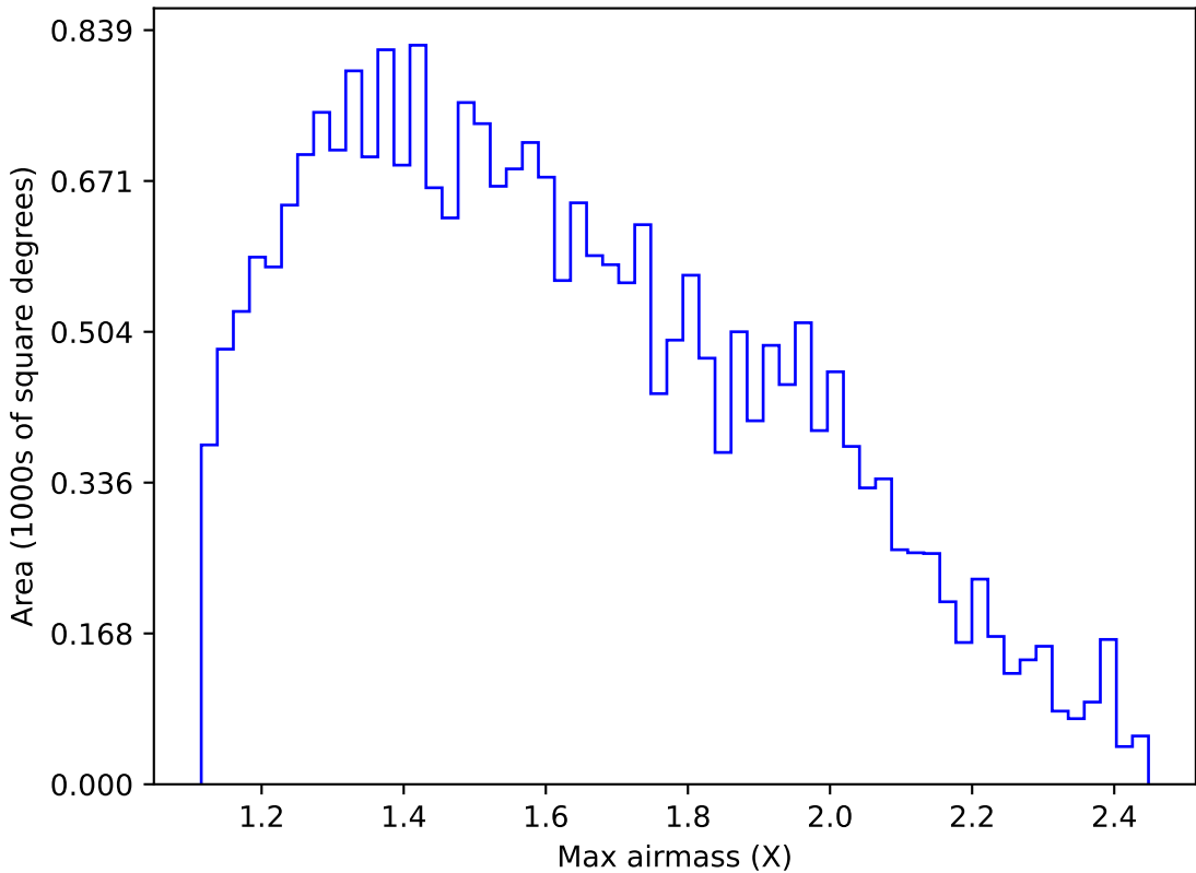
ddf_acor_sf10_lsf40_lsr10_v3.4_10yrs Yr 1 g band: Max airmass
