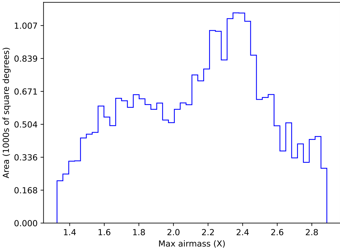
ddf_acor_sf10_lsf40_lsr10_v3.4_10yrs Yr 1 all bands: Max airmass
