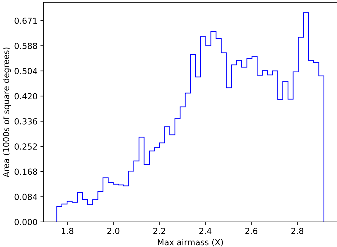
ddf_acor_sf10_lsf40_lsr10_v3.4_10yrs WFD z band: Max airmass
