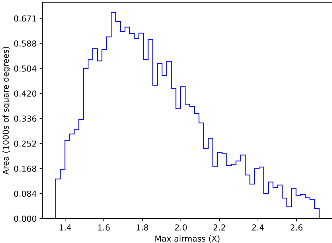
ddf_acor_sf10_lsf40_lsr10_v3.4_10yrs WFD u band: Max airmass
