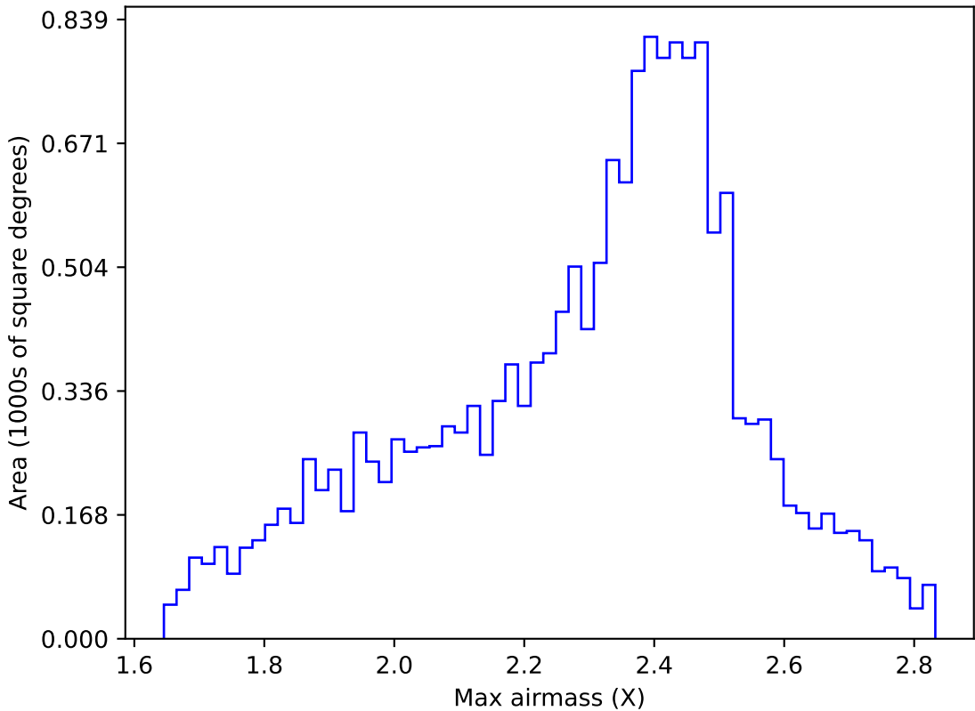
ddf_acor_sf10_lsf40_lsr10_v3.4_10yrs WFD r band: Max airmass
