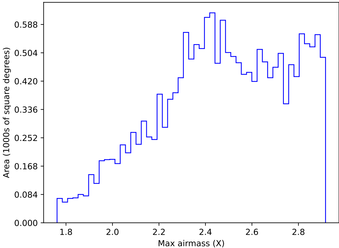
ddf_acor_sf10_lsf40_lsr10_v3.4_10yrs WFD i band: Max airmass
