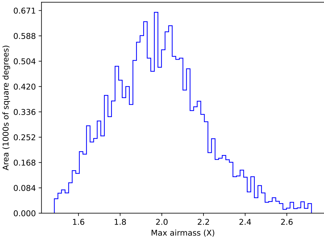
ddf_acor_sf10_lsf40_lsr10_v3.4_10yrs WFD g band: Max airmass
