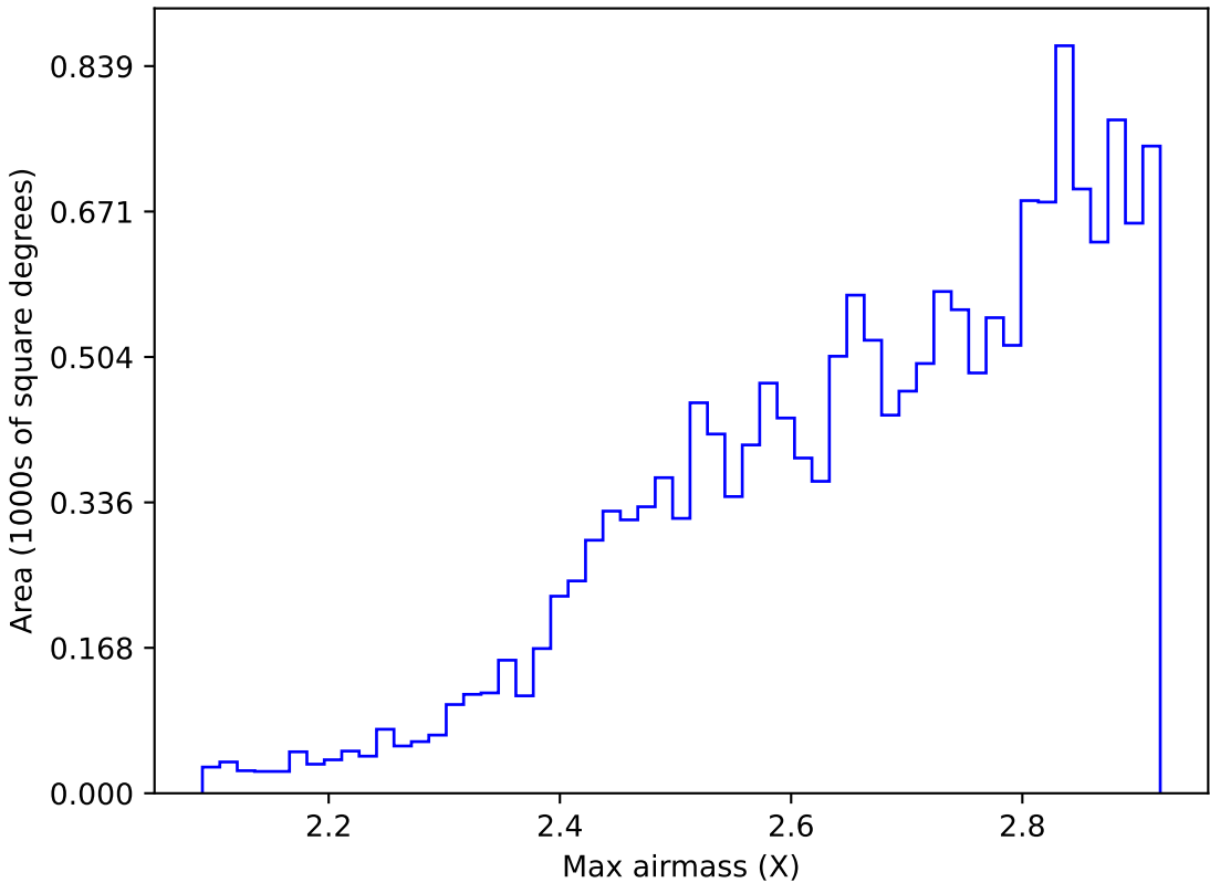
ddf_acor_sf10_lsf40_lsr10_v3.4_10yrs WFD all bands: Max airmass
