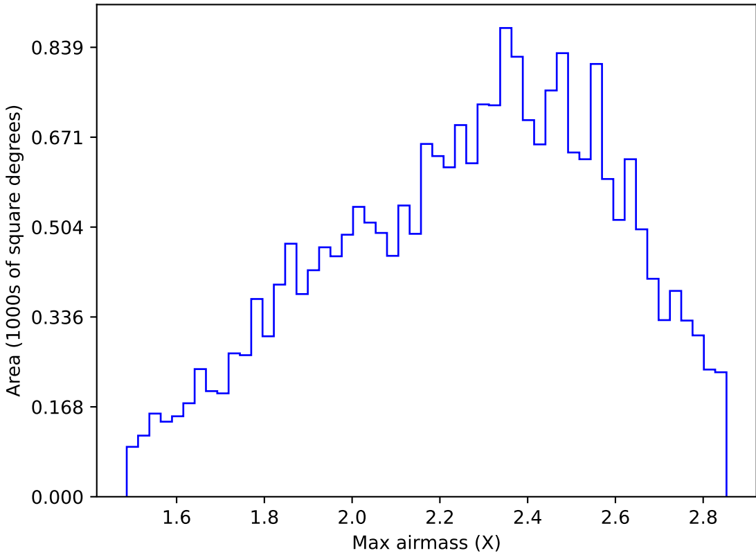
ddf_acor_sf10_lsf40_lsr10_v3.4_10yrs All sky y band: Max airmass
