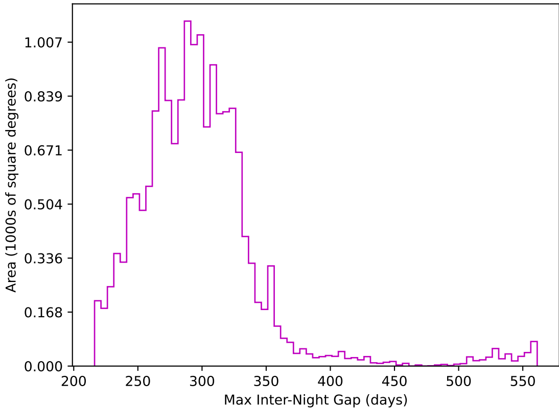
ddf_acor_sf10_lsf40_lsr10_v3.4_10yrs WFD z band: Max Inter-Night Gap
