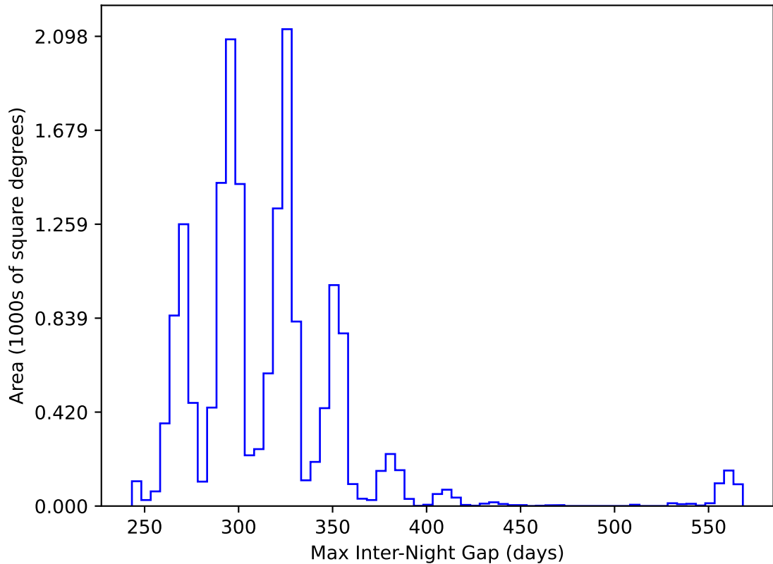
ddf_acor_sf10_lsf40_lsr10_v3.4_10yrs WFD y band: Max Inter-Night Gap
