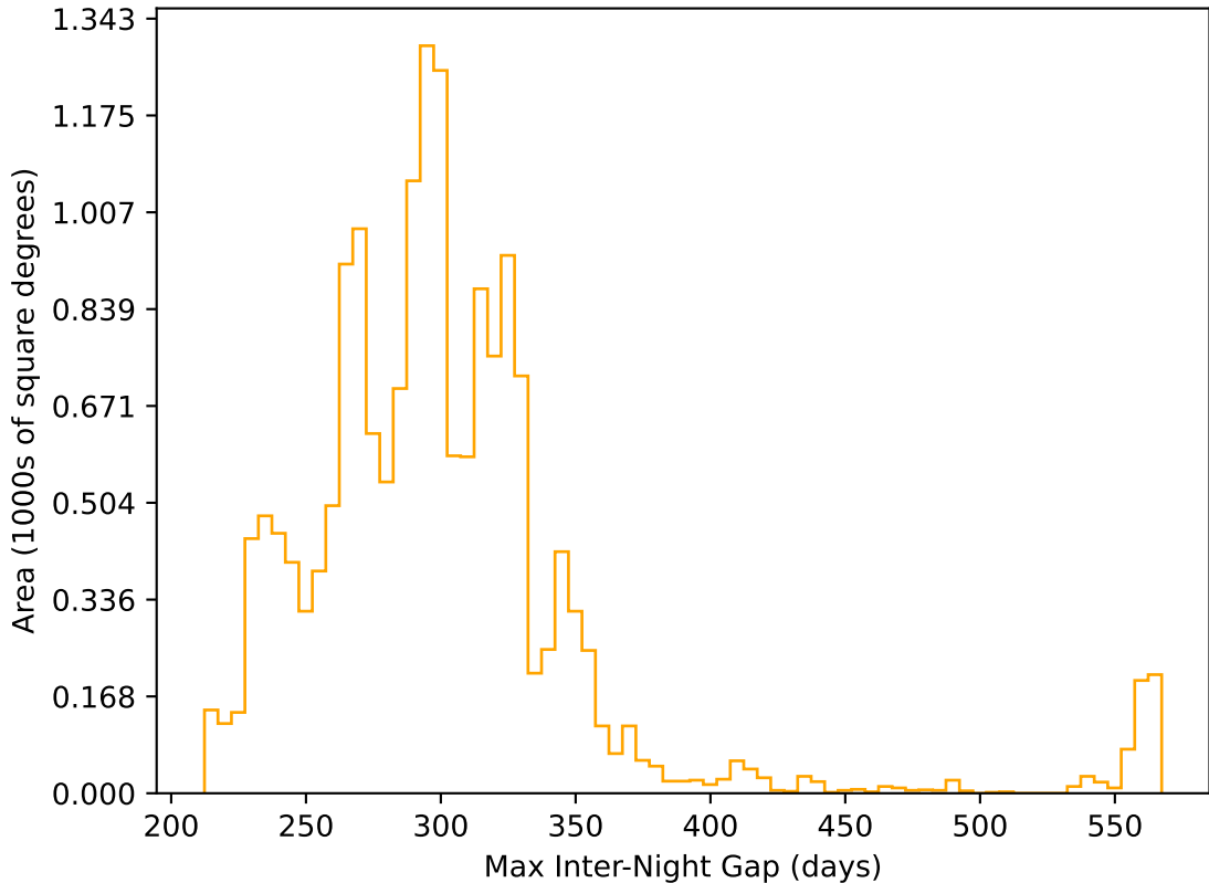
ddf_acor_sf10_lsf40_lsr10_v3.4_10yrs WFD r band: Max Inter-Night Gap
