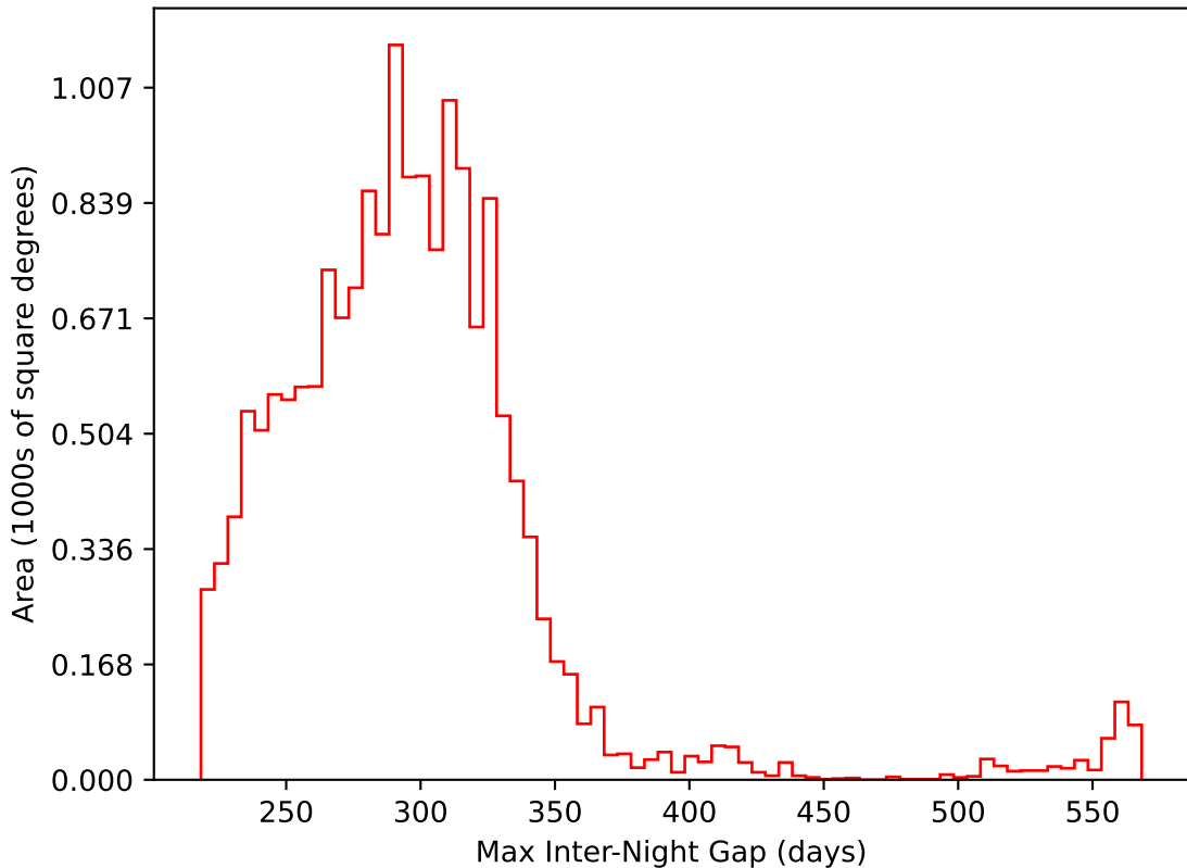
ddf_acor_sf10_ls40_lsr10_v3.4_10yrs WFD i band: Max Inter-Night Gap
