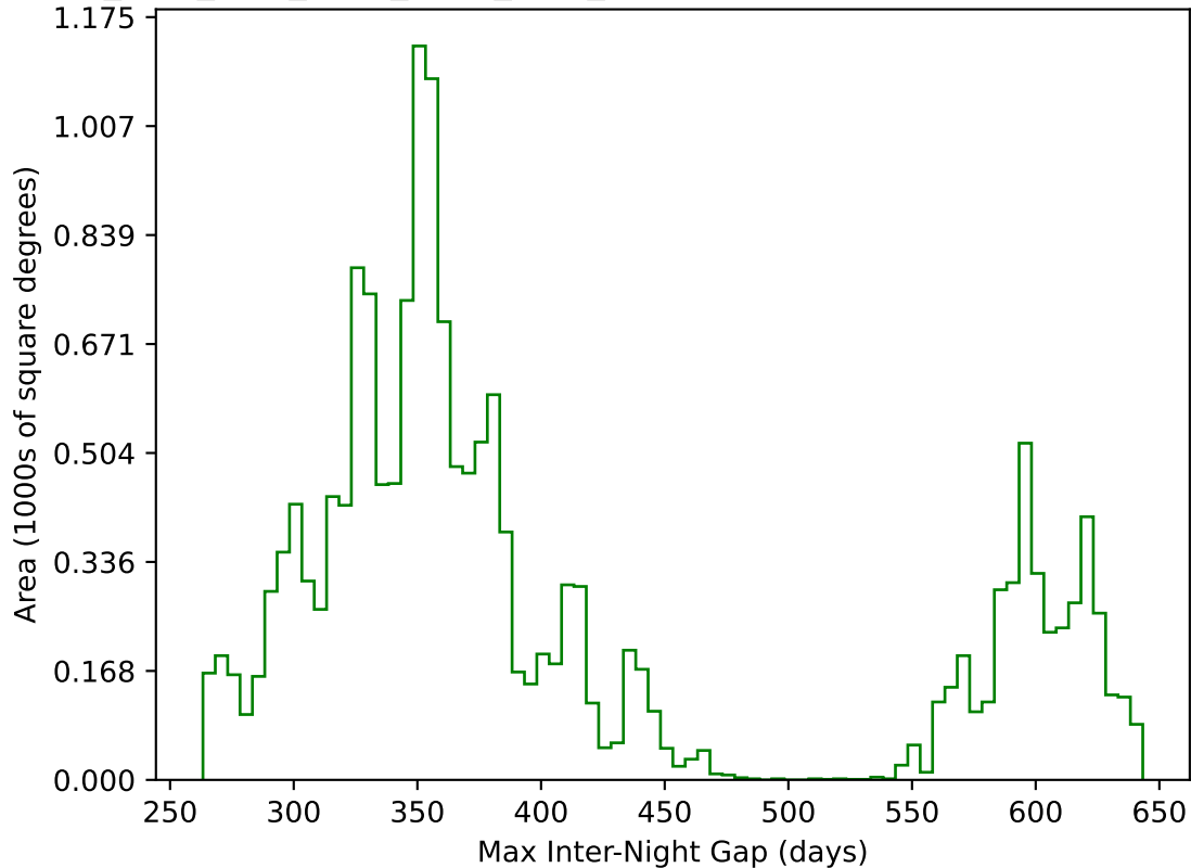
ddf_acor_sf10_lsf40_lsr10_v3.4_10yrs WFD g band: Max Inter-Night Gap
