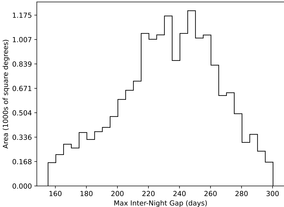
ddf_acor_sf10_lsf40_lsr10_v3.4_10yrs WFD all bands: Max Inter-Night Gap
