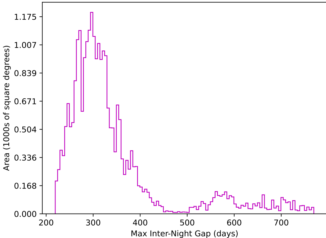
ddf_acor_sf10_lsf40_lsr10_v3.4_10yrs All sky z band: Max Inter-Night Gap
