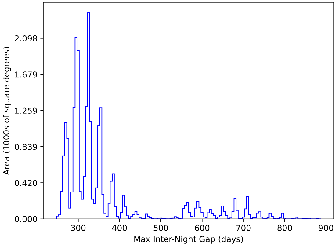
ddf_acor_sf10_lsf40_lsr10_v3.4_10yrs All sky y band: Max Inter-Night Gap
