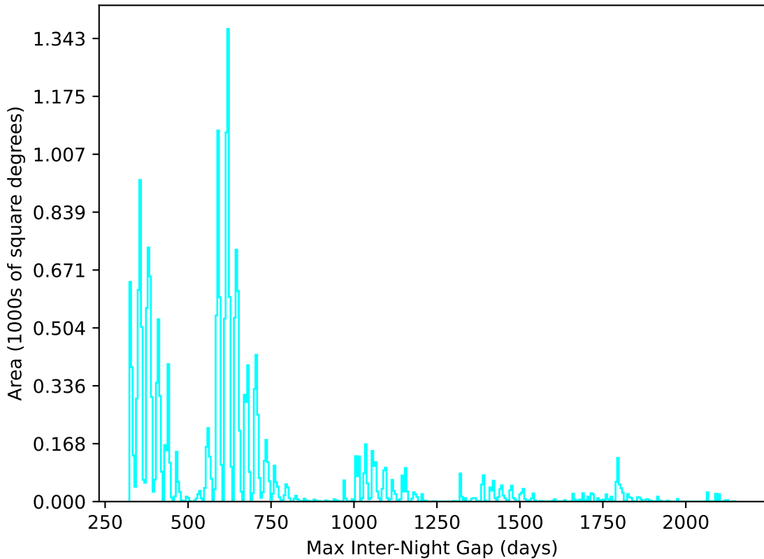
ddf_acor_sf10_lsf40_lsr10_v3.4_10yrs All sky u band: Max Inter-Night Gap
