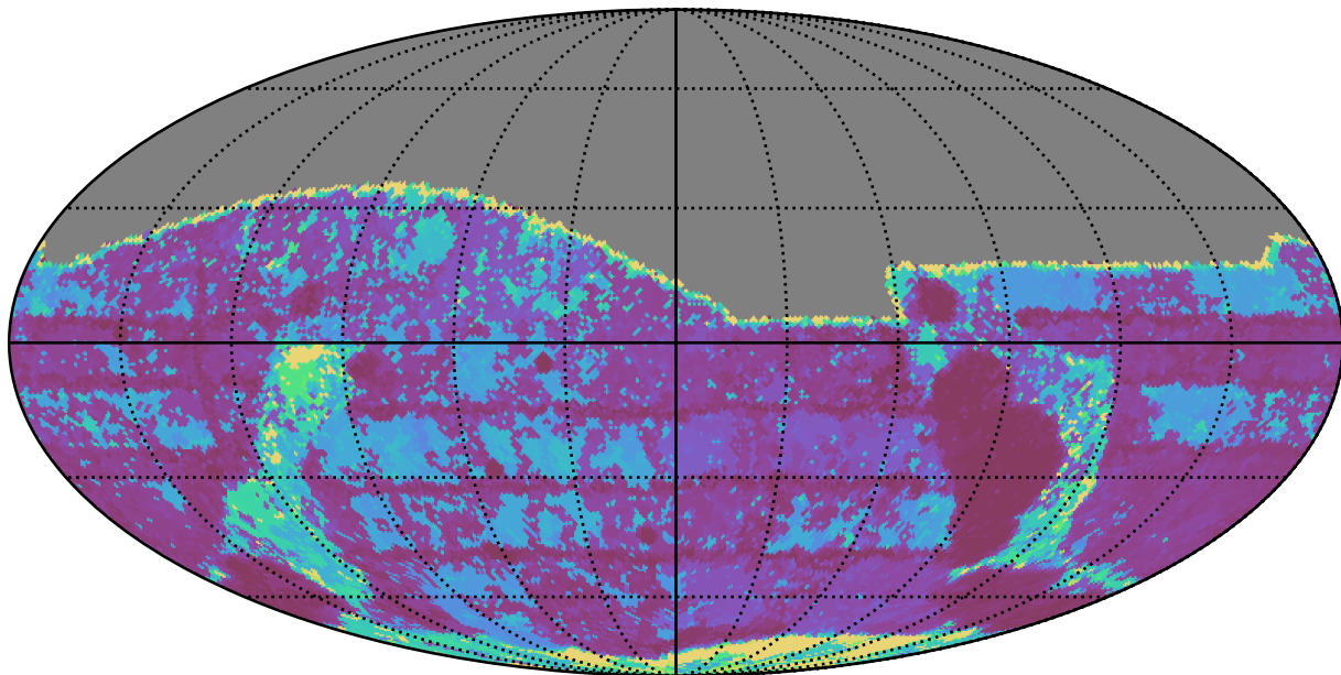
ddf_acor_sf10_lsf40_lsr10_v3.4_10yrs All sky g band: Max Inter-Night Gap
