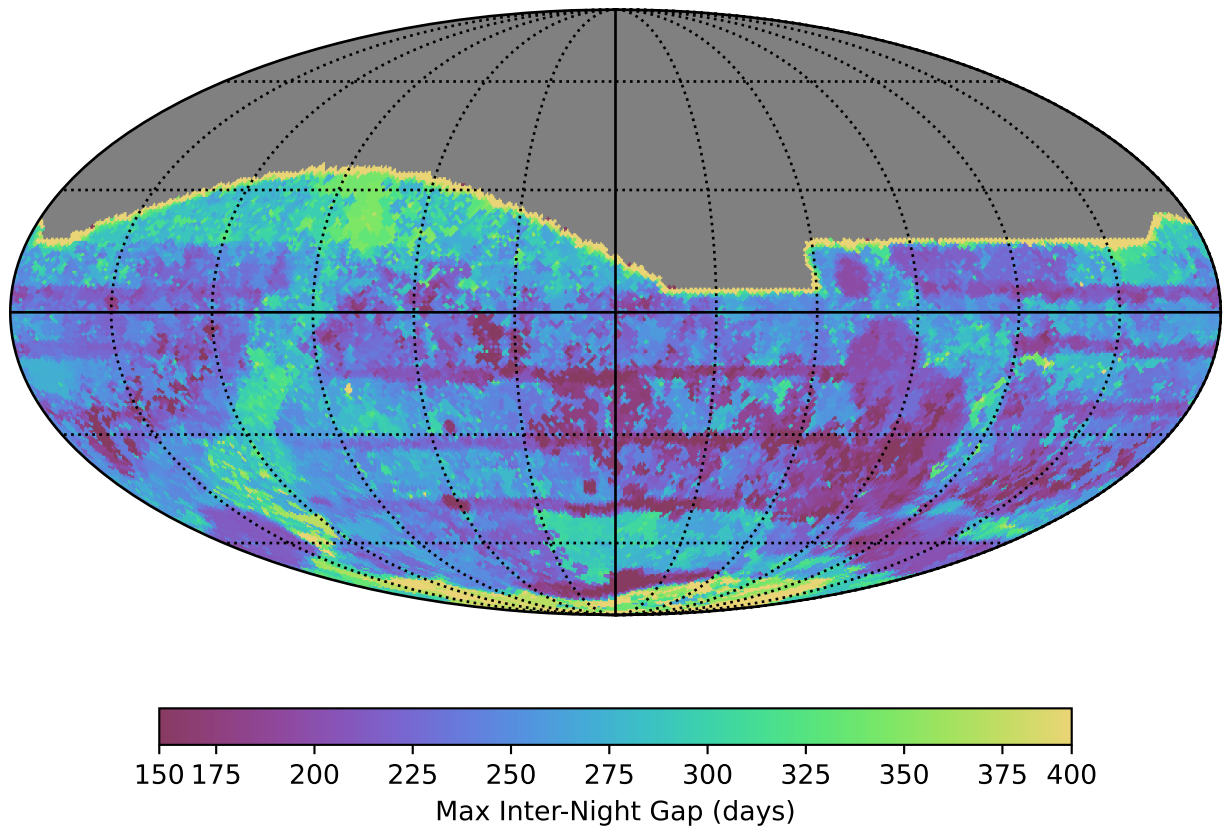
ddf_acor_sf10_lsf40_lsr10_v3.4_10yrs All sky all bands: Max Inter-Night Gap
