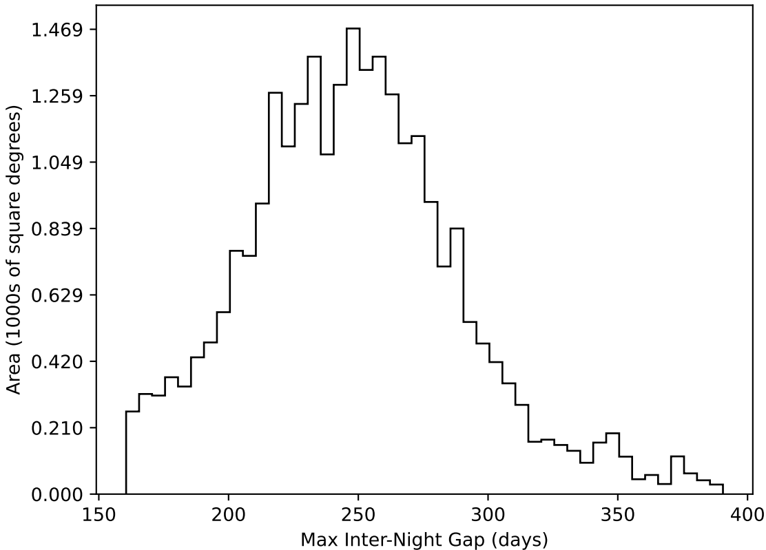
ddf_acor_sf10_lsf40_lsr10_v3.4_10yrs All sky all bands: Max Inter-Night Gap
