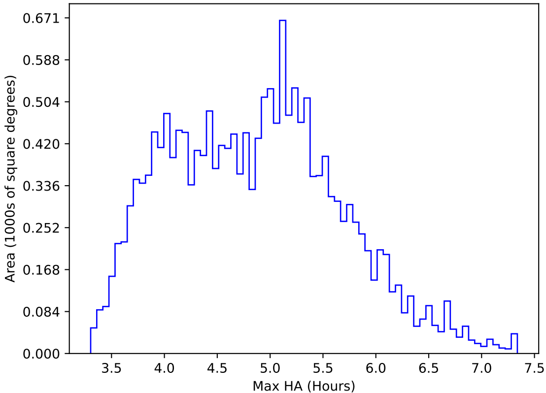
ddf_acor_sf10_lsf40_lsr10_v3.4_10yrs WFD z band: Max HA
