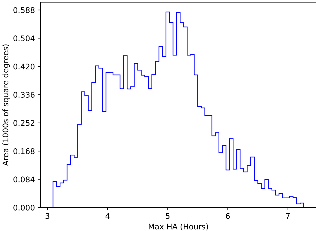
ddf_acor_sf10_lsf40_lsr10_v3.4_10yrs WFD i band: Max HA
