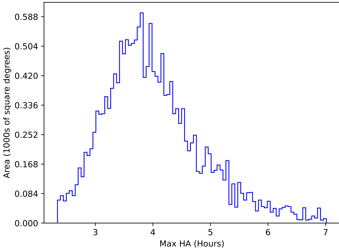
ddf_acor_sf10_lsf40_lsr10_v3.4_10yrs WFD g band: Max HA
