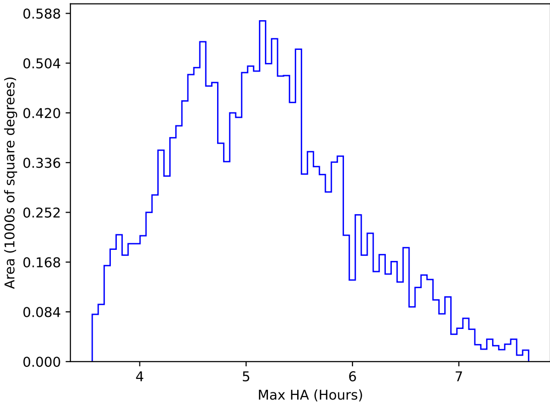
ddf_acor_sf10_lsf40_lsr10_v3.4_10yrs WFD all bands: Max HA
