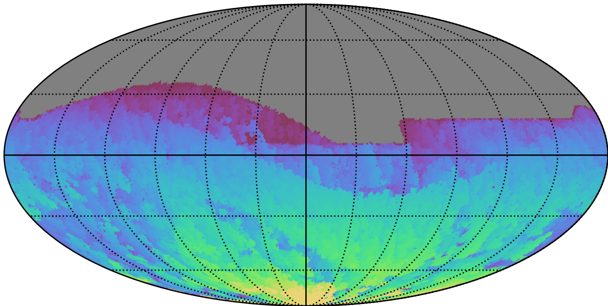
ddf_acor_sf10_lsf40_lsr10_v3.4_10yrs All sky z band: Max HA
