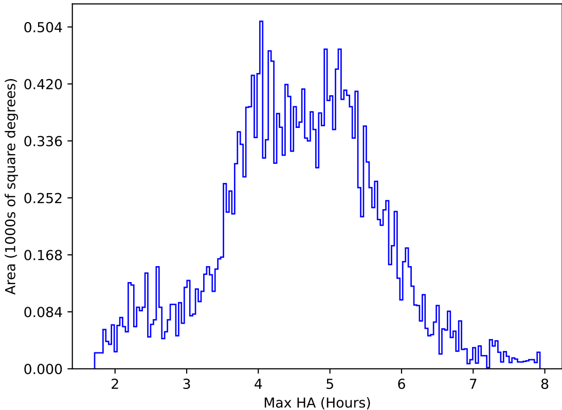
ddf_acor_sf10_ls40_lsr10_v3.4_10yrs All sky z band: Max HA
