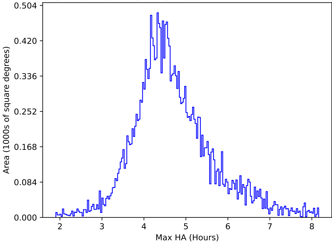
ddf_acor_sf10_ls40_lsr10_v3.4_10yrs All sky y band: Max HA
