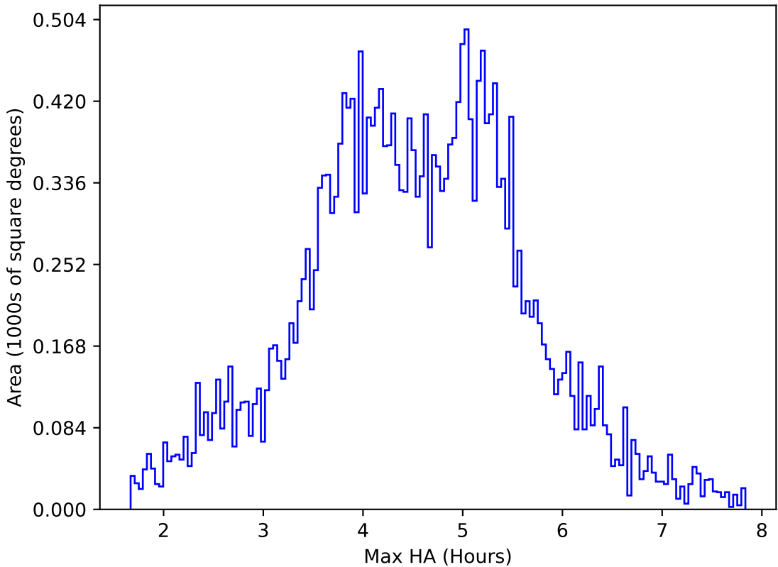
ddf_acor_sf10_lsf40_lsr10_v3.4_10yrs All sky i band: Max HA
