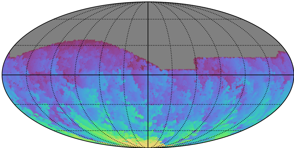
ddf_acor_sf10_lsf40_lsr10_v3.4_10yrs All sky g band: Max HA
