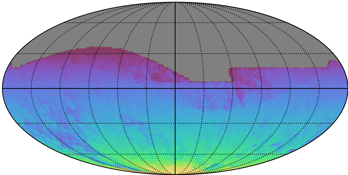
ddf_acor_sf10_lsf40_lsr10_v3.4_10yrs All sky all bands: Max HA
