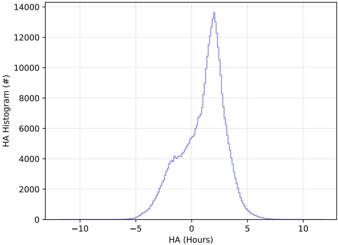
ddf_acor_sf10_lsf40_lsr10_v3.4_10yrs WFD y band: HA Histogram
