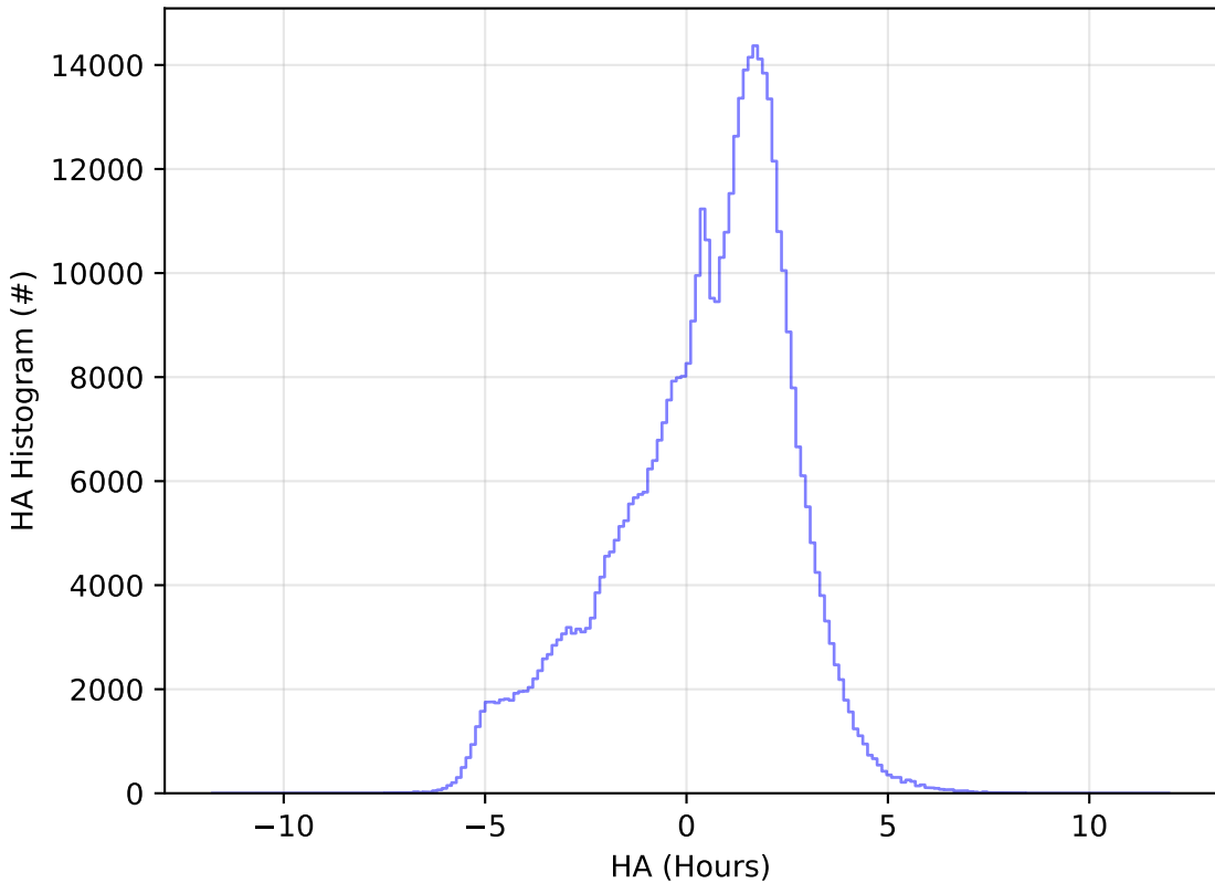
ddf_acor_sf10_lsf40_lsr10_v3.4_10yrs WFD r band: HA Histogram
