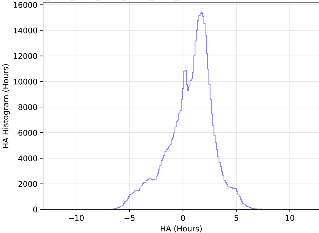
ddf_acor_sf10_ls40_lsr10_v3.4_10yrs WFD i band: HA Histogram
