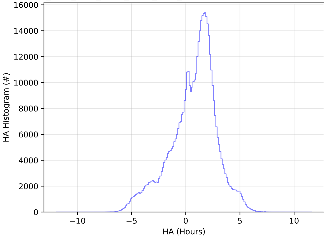
ddf_acor_sf10_lsf40_lsr10_v3.4_10yrs WFD i band: HA Histogram
