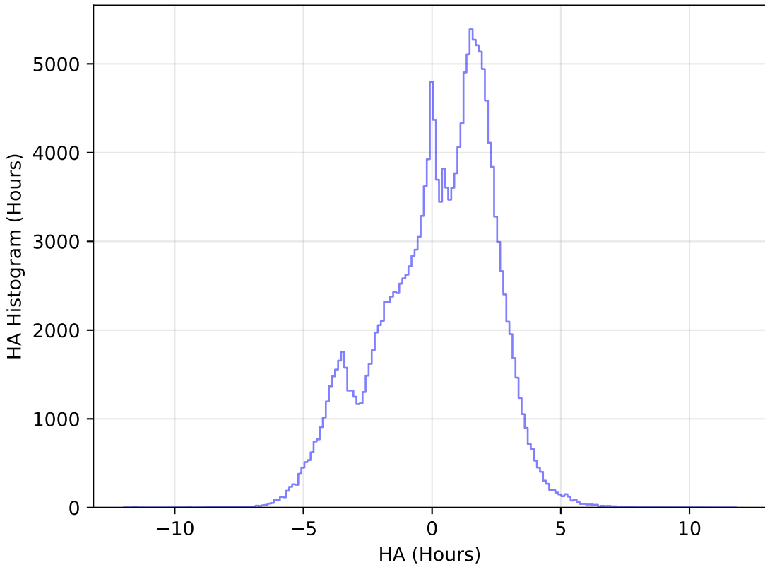
ddf_acor_sf10_lsf40_lsr10_v3.4_10yrs WFD g band: HA Histogram
