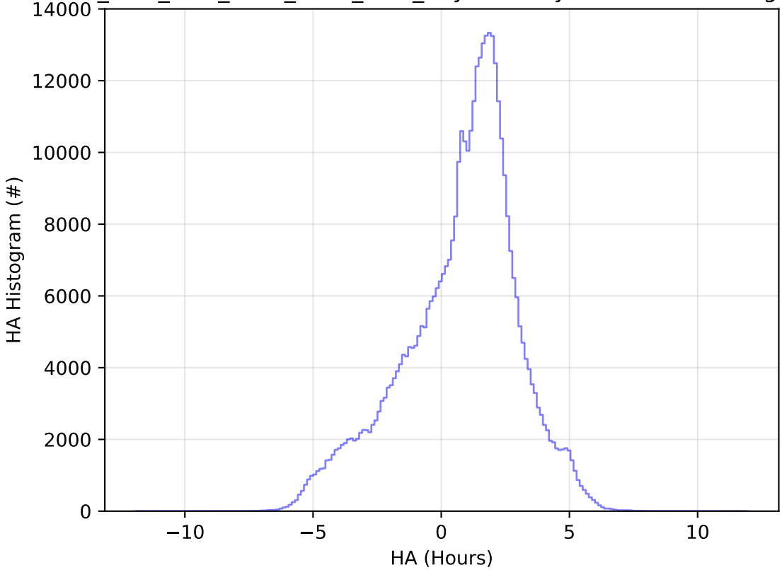
ddf_acor_sf10_lsf40_lsr10_v3.4_10yrs All sky z band: HA Histogram
