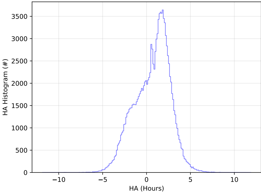
ddf_acor_sf10_lsf40_lsr10_v3.4_10yrs All sky u band: HA Histogram
