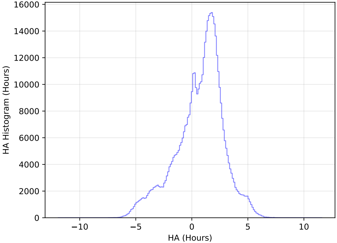
ddf_acor_sf10_lsf40_lsr10_v3.4_10yrs All sky i band: HA Histogram
